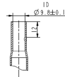
吐出管详细 DISCHARGE TUBE
