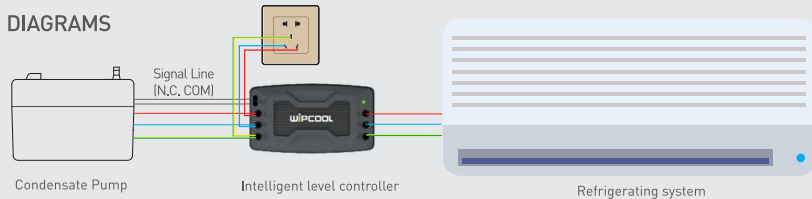
Failure drainage status-Output was cut off when water reaches alarm level to trigger safety switch, To prevent refrigeration equipment continues to generating the condensate water
